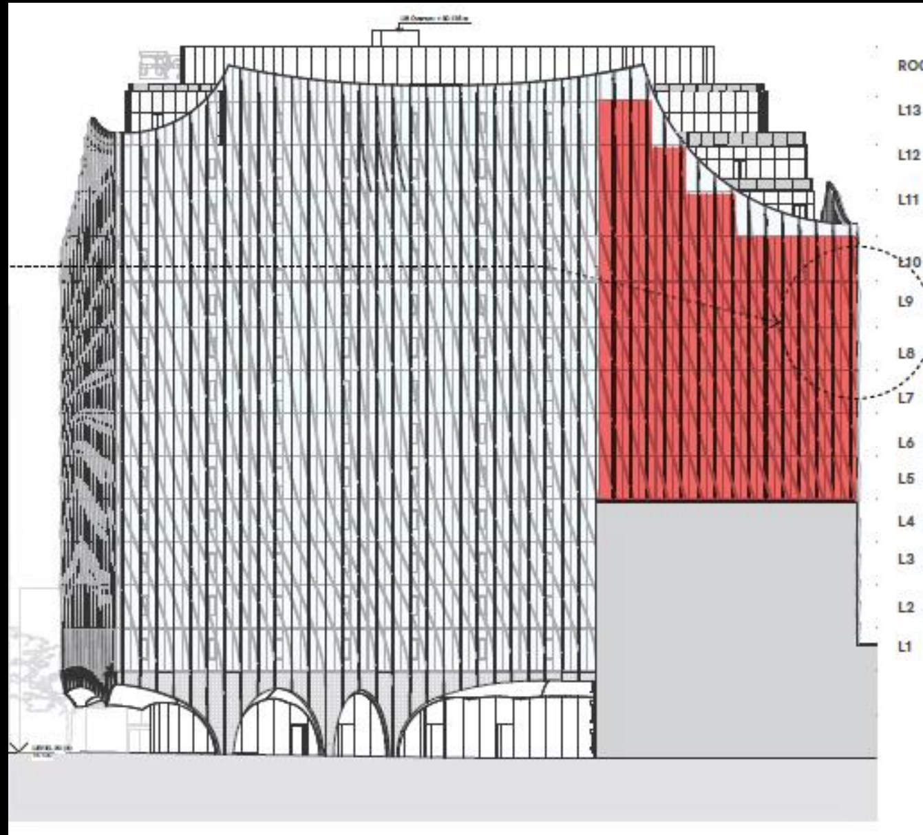
East Elevations – Party Wall Revisions
