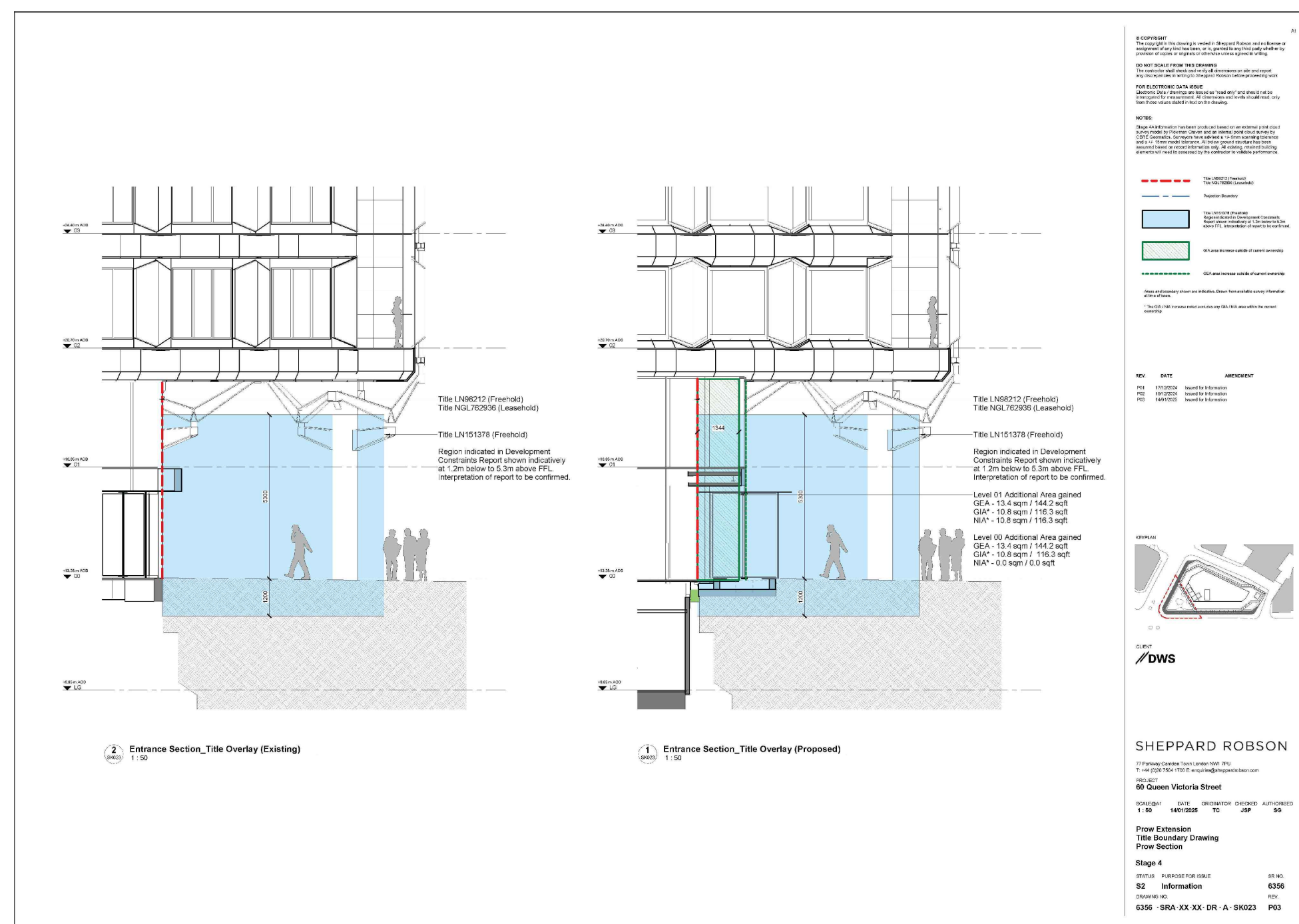
Extract of Sheppard Robson elevational plan Drawing no. 6356-SRA-XX-XX-DR-A-SK023 Rev P03 Proposed Entrance Area Ground Floor Not to Scale
