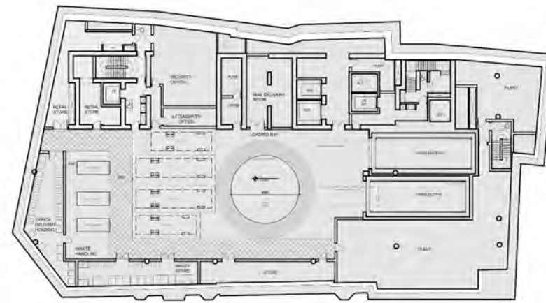
2 PROPOSED BASEMENT 1
