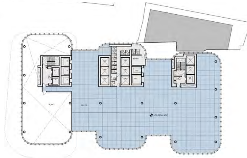
2 PROPOSED LEVEL 06 PLAN
