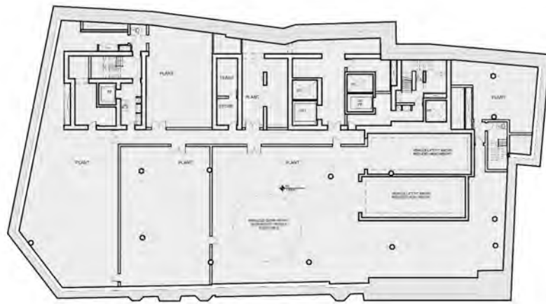
1 PROPOSED BASEMENT 2
