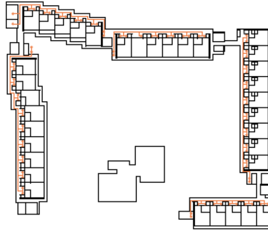
Level 4 Plan - Pipe Distribution
