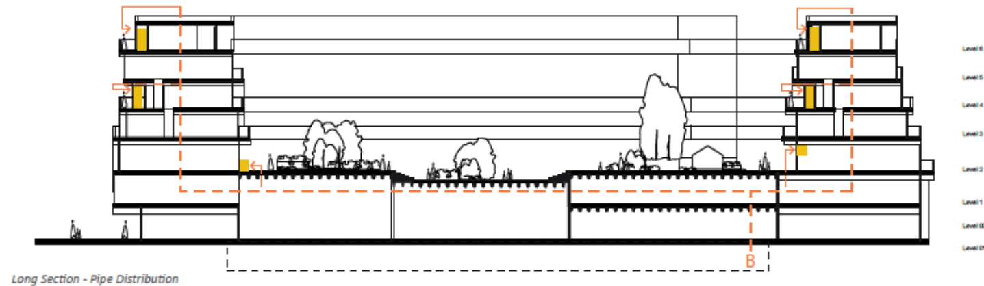
Long Section - Pipe Distribution
