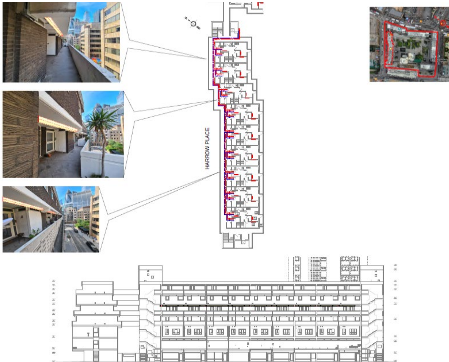
Harrow Place external facing 4 th floor proposed heating distribution system
